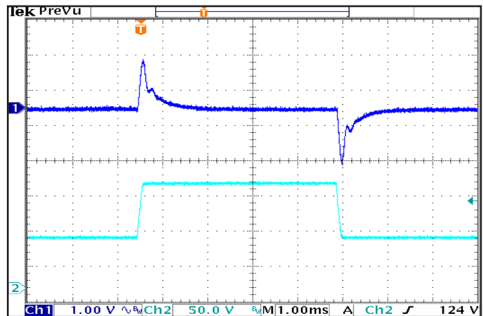
Figure 6: Output voltage response to step-change in input voltage (1V/ms). Load cap: 1 μF ceramic capacitor. Ch 1: V out , Ch 2: V in .
